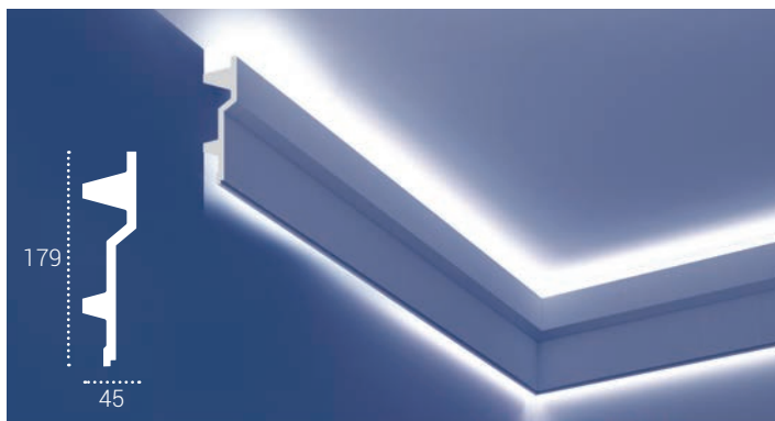
KF 707 | 179x45mm
